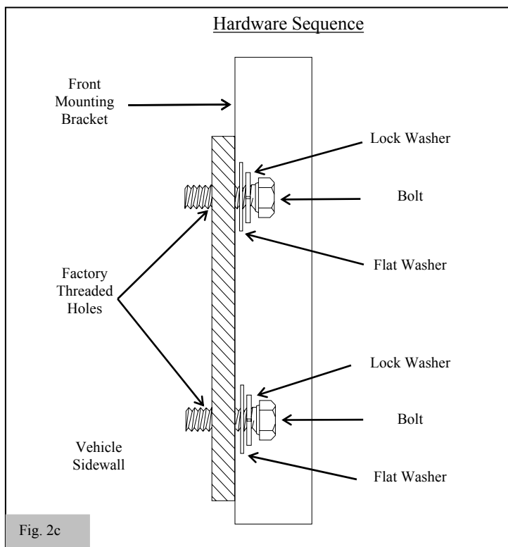
Driver and Passenger brackets shown in above picture / 4 brackets per side.
